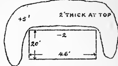
C PLAN OF SHELTER 70 YDS IN REAR OF PARAPET
